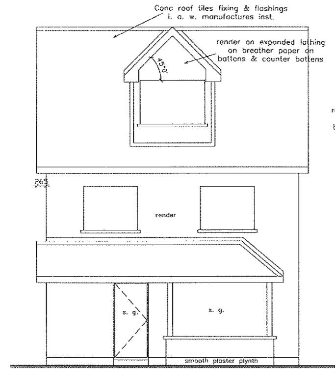
Rear Elevation
