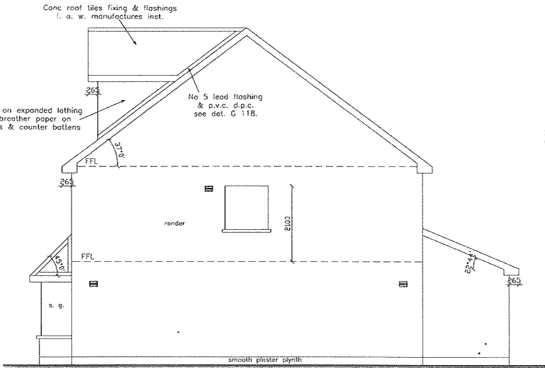
Side Elevation
